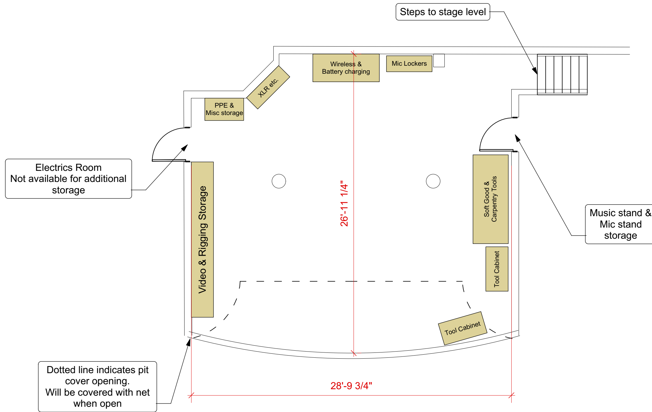
1 Orchestra Pit Schematic Layout Scale: 3/16" = 1'-0"
